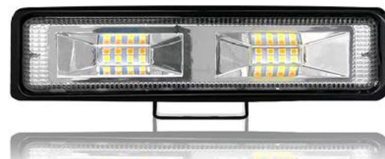
XK-16LED-WYF AC/DC 8V-80V 48W/4800LM
